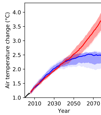
Figure 2: Projections of air temperature for all of Pakistan for different GHG emissions scenarios.
