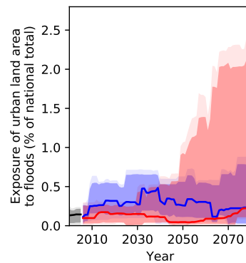
Figure 23: Projections of urban land area exposed to river floods at least once a year for all of Pakistan for different GHG emissions scenarios.
